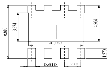
DIMENSIONS:MILLIMETERS
